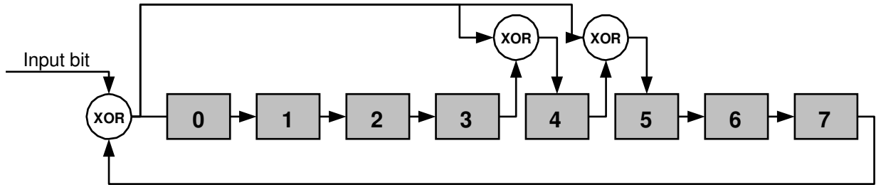
Figure 1 Internal structure of the RHTSxx CRC-8 generator
