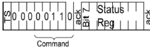
Figure 7 Status Register Write
