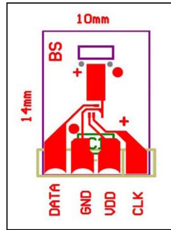
SMD package
