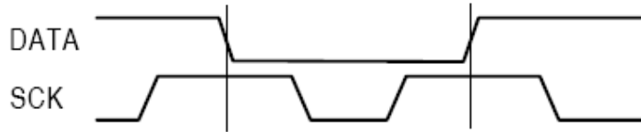
Figure 3 "Transmission Start" sequence
