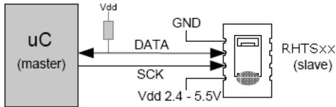
Figure 2 Typical application circuit
