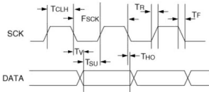
Figure 9 Timing Diagram
